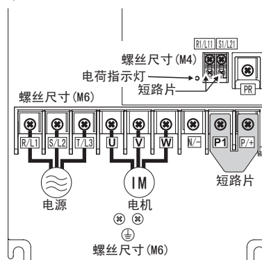
FR-F740-22K, 30K-CH
