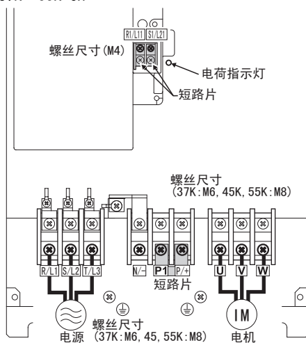
FR-F740-37K~55K-CH
