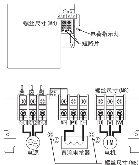
FR-F740-S75K-CH
