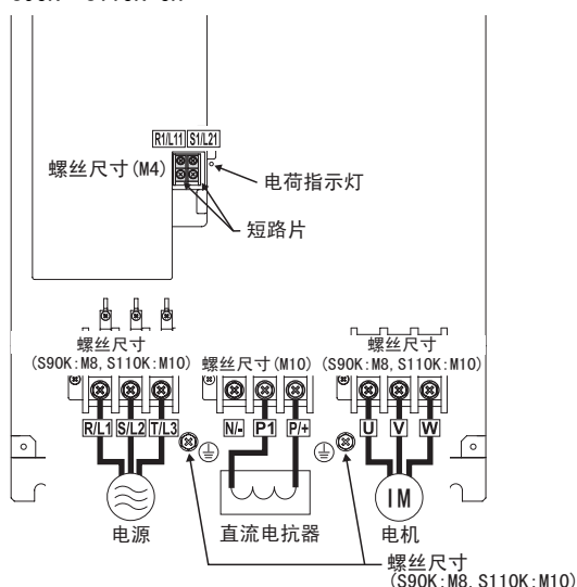
FR-F740-S90K~S110K-CH
