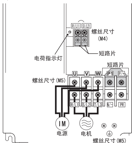
FR-F740-15K, 18.5K-CH
