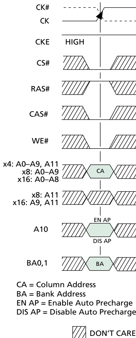
Figure 14 WRITE Command
