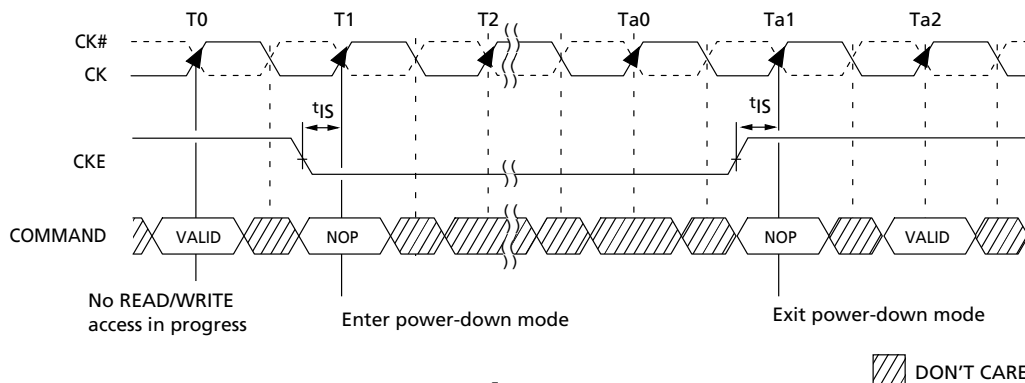
Figure 26 Power-Down
