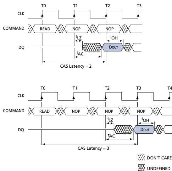
Figure 8: CAS Latency
