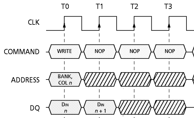
Figure 14 WRITE Burst
