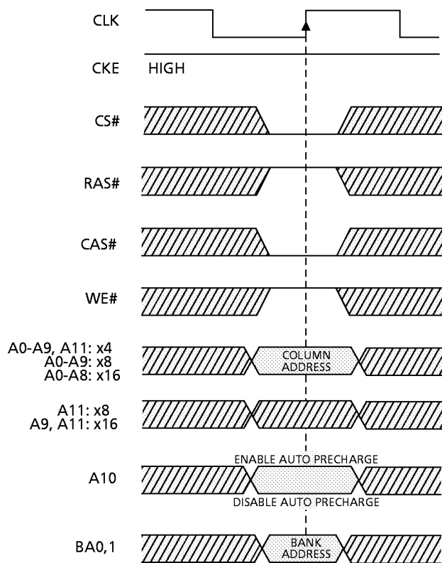
Figure 5 READ Command
