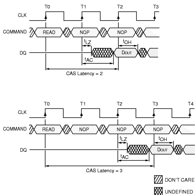
Figure 6 CAS Latency
