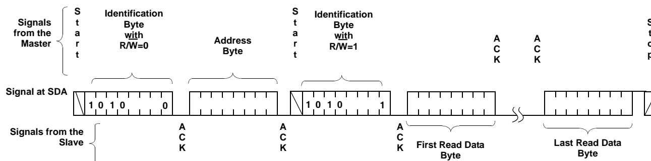
FIGURE 18. READ SEQUENCE
