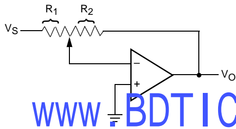
Inverting Amplifier
