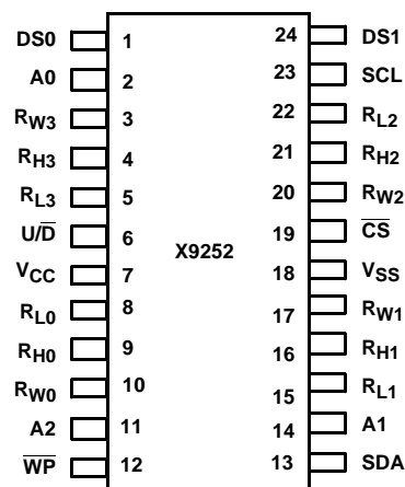
X9252 (24 LD SOIC/TSSOP) TOP VIEW
