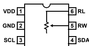
ISL90726 (6 LD SC-70) TOP VIEW
