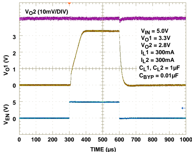
FIGURE 14. TURN-ON/TURN-OFF RESPONSE
