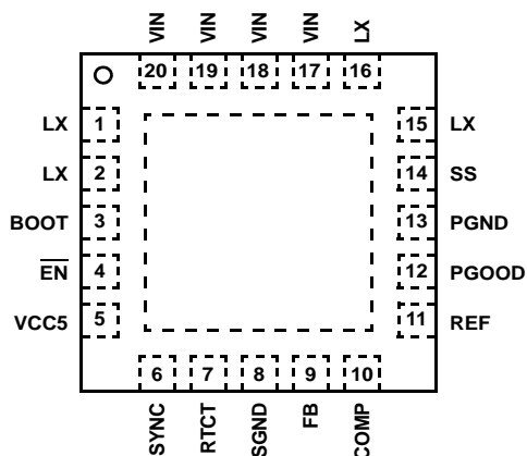
ISL8560MREP (20 LD QFN) TOP VIEW
