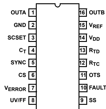
ISL6740A (TSSOP) TOP VIEW
