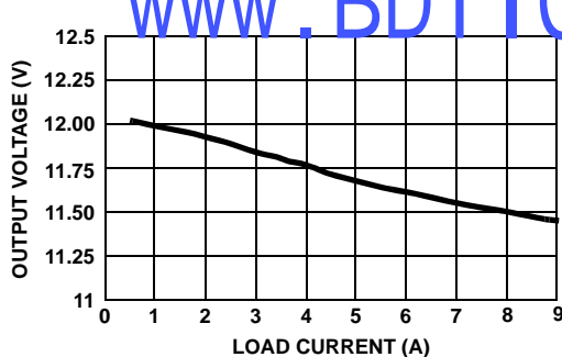
FIGURE 11. LOAD REGULATION AT V_{IN} = 48V
