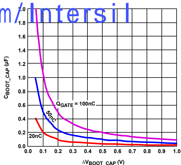
FIGURE 8. BOOTSTRAP CAPACITANCE vs BOOT RIPPLE VOLTAGE
