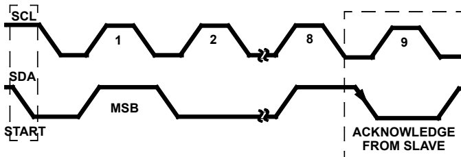
FIGURE 3. ACKNOWLEDGE ON THE I²C BUS
