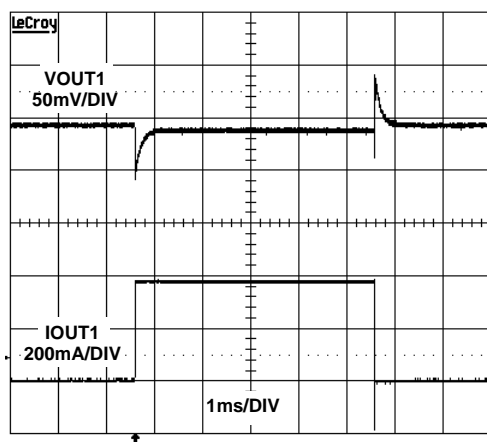
FIGURE 4. LDO1 TRANSIENT RESPONSE (10mA to 330mA)
