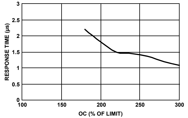
FIGURE 10. RESPONSE TIME vs I_O \cdot R_{\text{SNS}}
