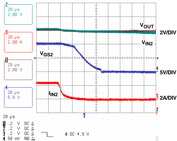
FIGURE 14. SLOW SPEED TURN-OFF, V_{IN} = 12V , COMMON LOAD IS SMPS ( C_{LOAD} = 100\mu F ) WITH EQUIVALENT 4A LOAD
