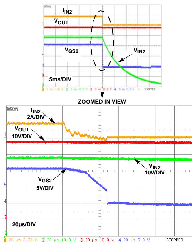
FIGURE 25. SLOW SPEED TURN-OFF ( C_{GSTOT} = 8.4nF + 33nF )
