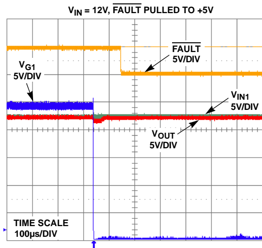
FIGURE 28. MOSFET GATE TO SOURCE FAULT
