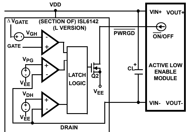
FIGURE 34. ACTIVE LOW ENABLE MODULE
