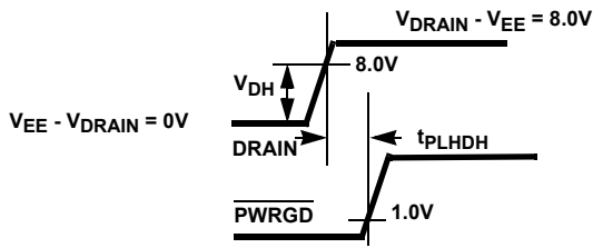
FIGURE 6A. DRAIN HIGH TO \overline{PWRGD} (INACTIVE) HIGH (ISL6142)
