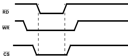
FIGURE 30. READ CYCLE
