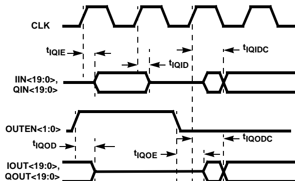
FIGURE 22. ENABLE/DISABLE TIMING
