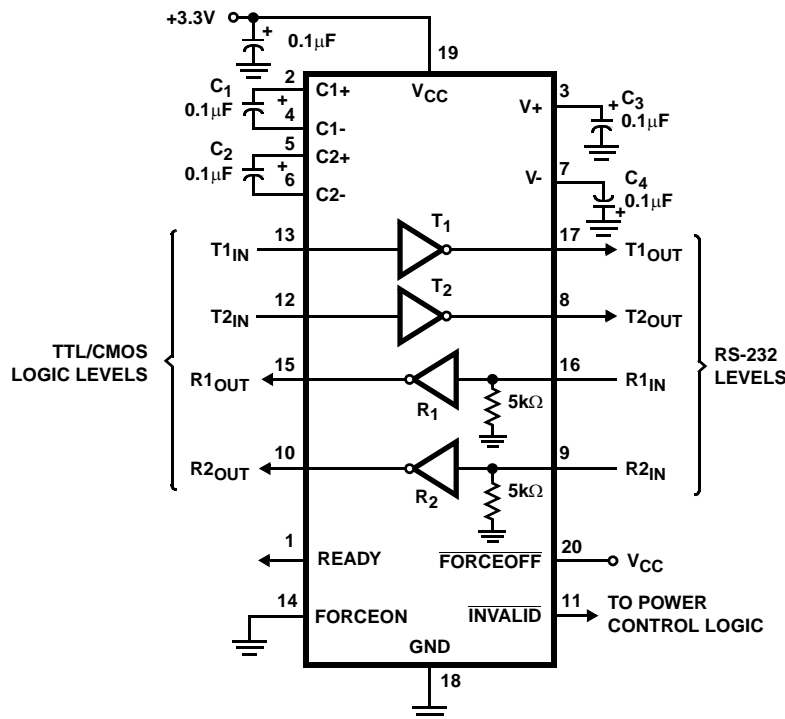
ICL3225
