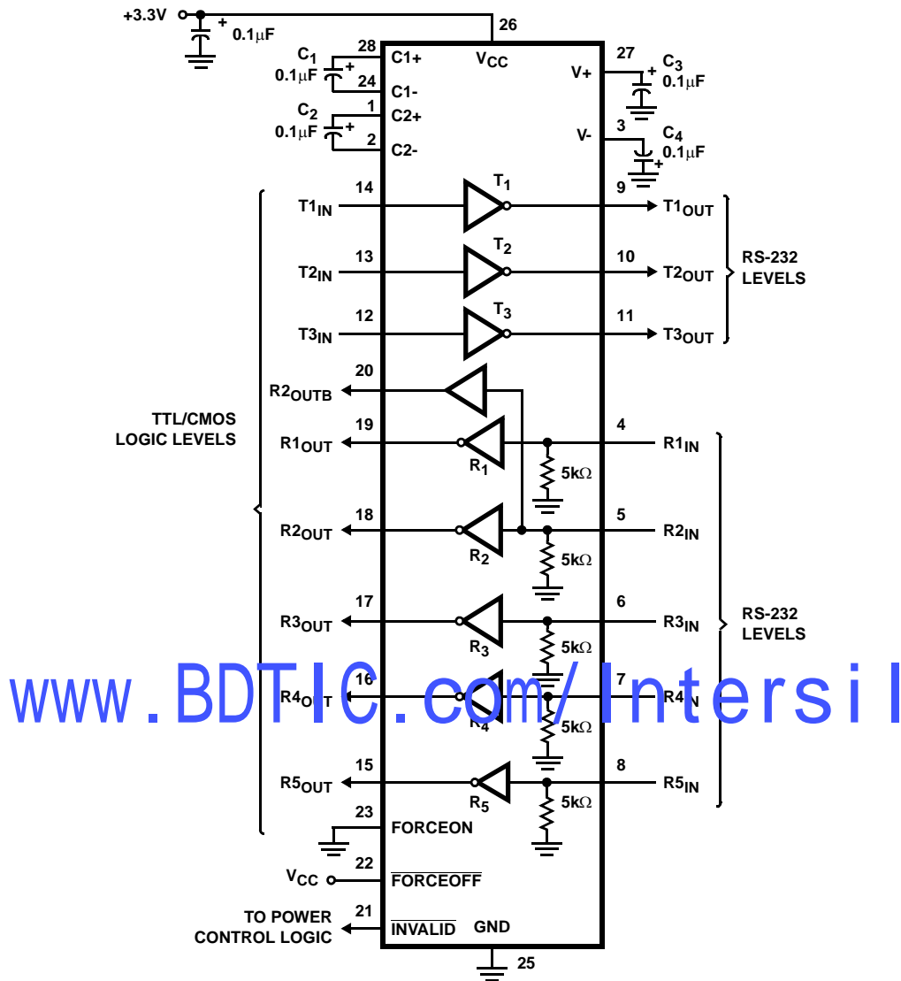
ICL3245
