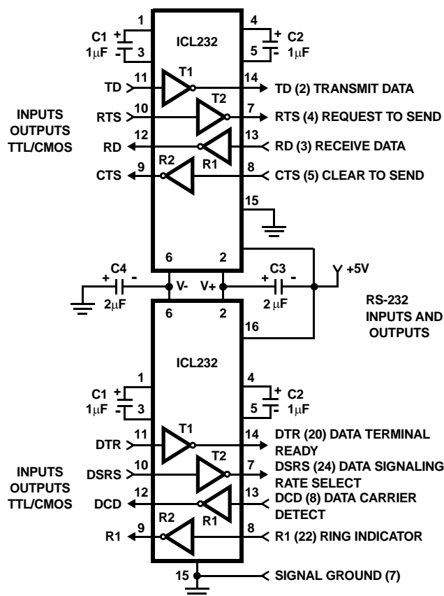
FIGURE 11. COMBINING TWO ICL232s FOR A PAIR OF RS-232 INPUTS AND OUTPUTS
