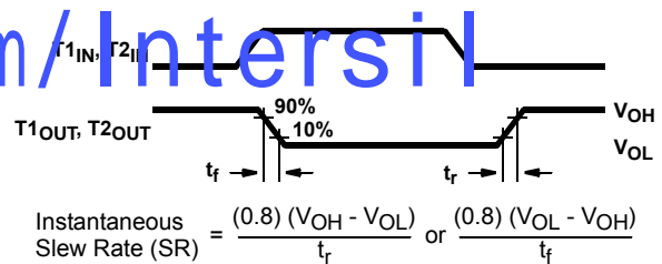
FIGURE 6. SLEW RATE DEFINITION
