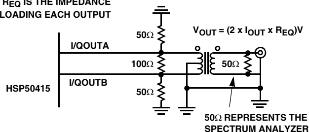
FIGURE 19. DAC OUTPUTS
