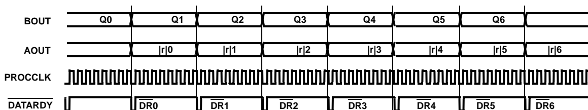
FIGURE 32. \overline{\text{DATARDY}} WAVEFORMS WHEN |r| (MAGNITUDE) IS SELECTED AS \text{AOUT}
