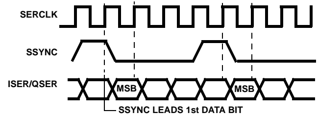
FIGURE 2. SERIAL INPUT TIMING FOR SER AND QSER INPUTS
