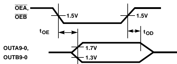
FIGURE 29. OUTPUT ENABLE/DISABLE
