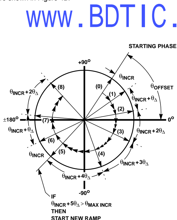
FIGURE 4A. PHASE WORD DURING UP CHIRP
