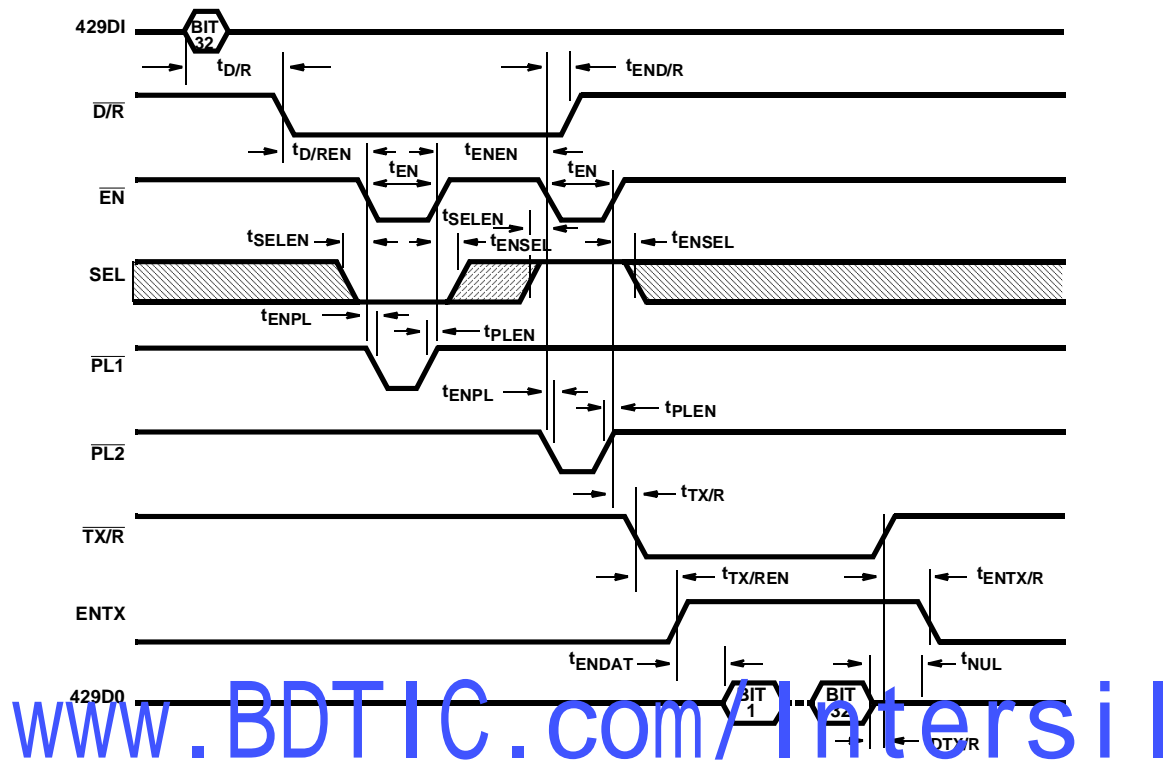
FIGURE 7. REPEATER OPERATION TIMING
