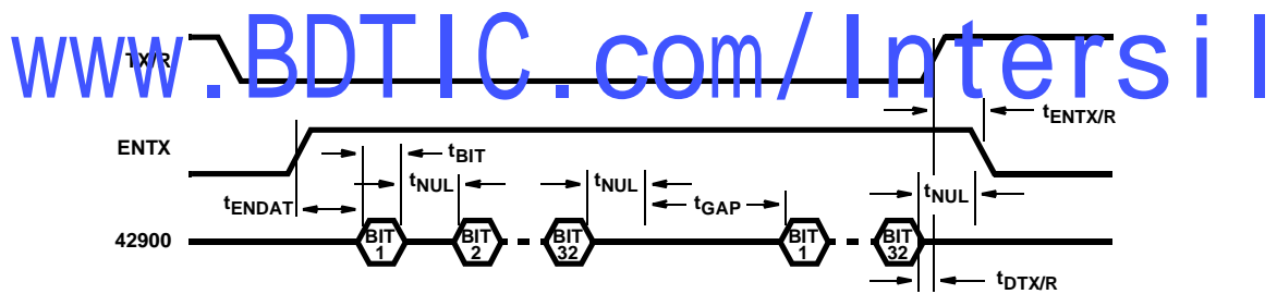
FIGURE 6. TRANSMITTER OUTPUT TIMING
