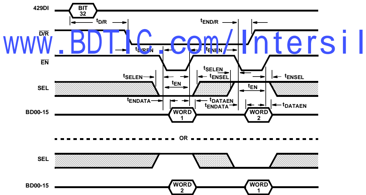
FIGURE 3. RECEIVER TIMING
