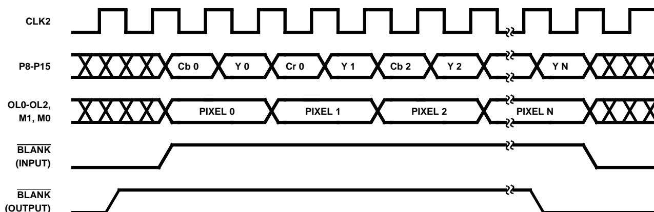
FIGURE 1. PIXEL AND OVERLAY INPUT TIMING - NORMAL 8-BIT YCbCr
