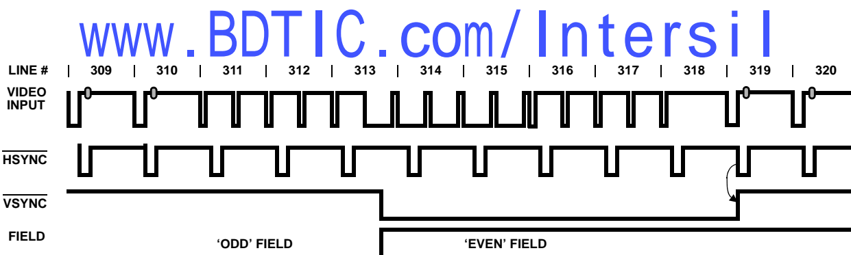
FIGURE 6. PAL(B, D, G, H, I, N, N C ) EVEN FIELD TIMING
