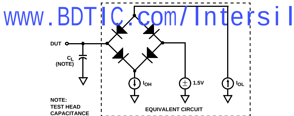
FIGURE 2. TEST CIRCUIT
