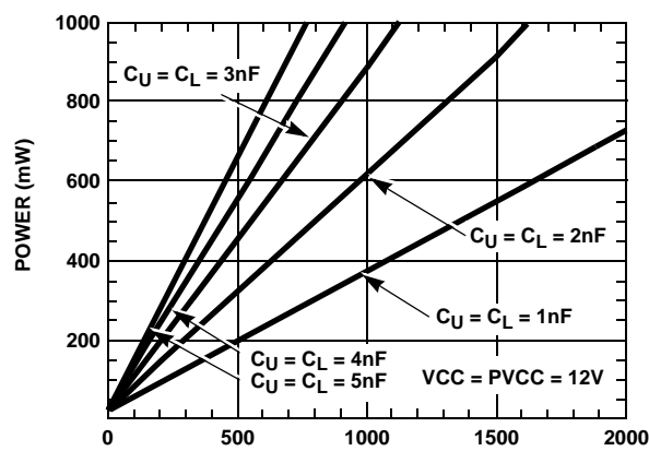
FIGURE 1. POWER DISSIPATION vs FREQUENCY
