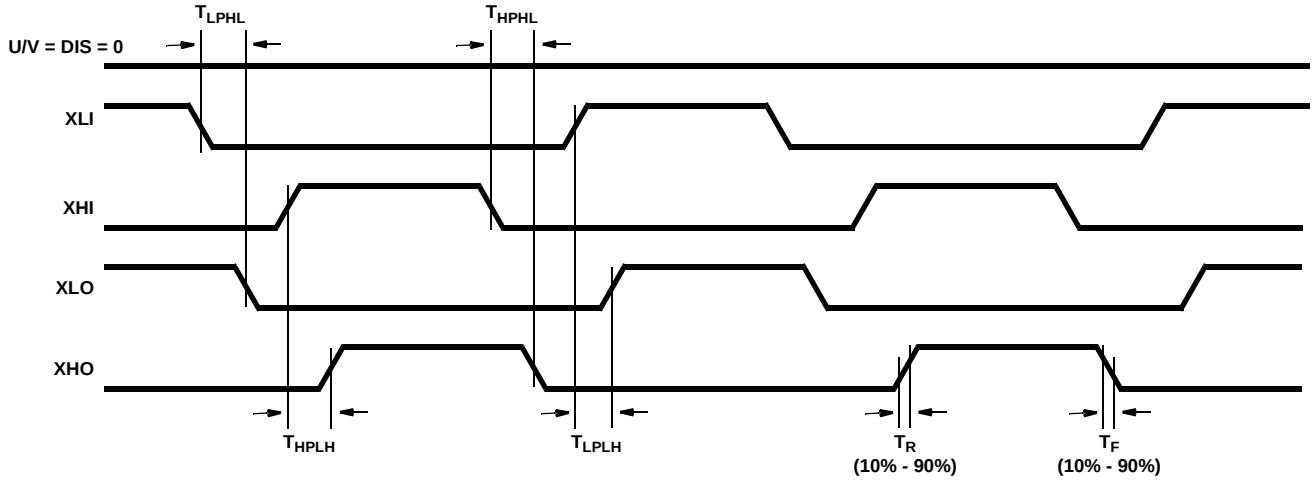
FIGURE 1. INDEPENDENT MODE
