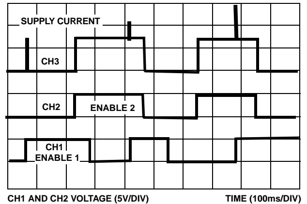
FIGURE 19. HIP1011DEVAL1 3.3V SUPPLY CURRENT AS CONTROLLER 1 TURNS ON INTO SHORTED LOAD CARD
