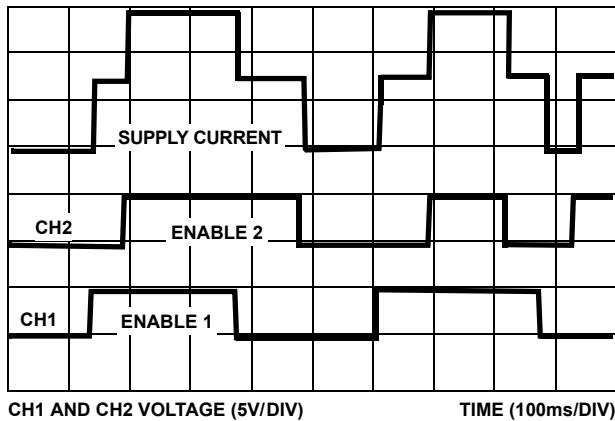
FIGURE 18. HIP1011DEVAL1 3.3V SUPPLY CURRENT AS EACH SLOT CONTROLLER TURNS ON INTO LOAD CARD
