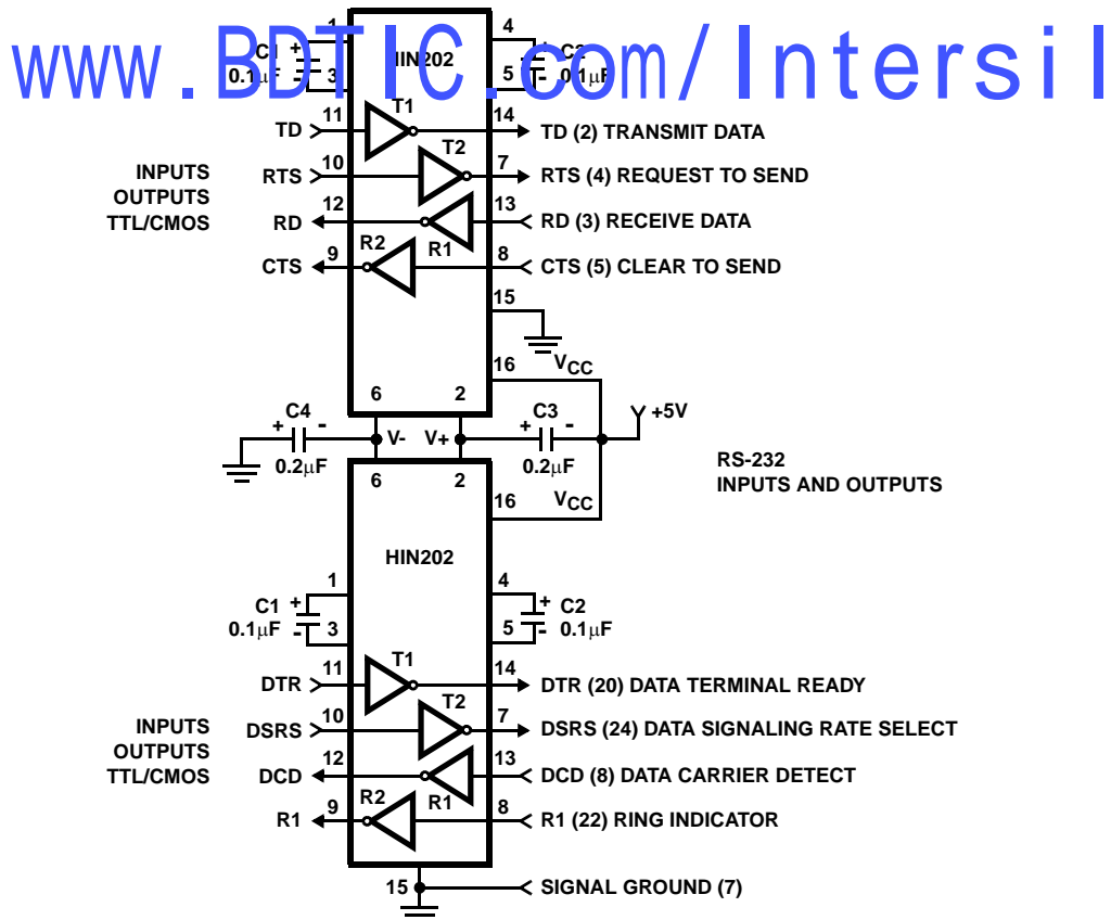
FIGURE 10. COMBINING TWO HIN202s FOR 4 PAIRS OF RS-232 INPUTS AND OUTPUTS
