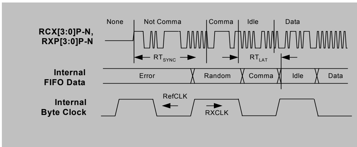
FIGURE 12. BYTE SYNCHRONIZATION
