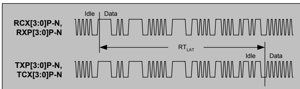
FIGURE 14. RETRANSMIT LATENCY
