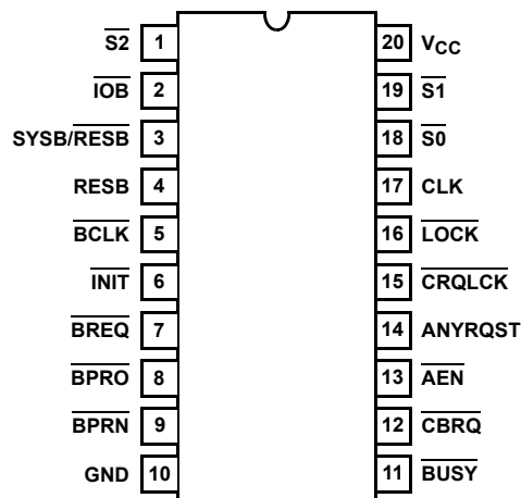
82C89 (PDIP, Cerdip)
