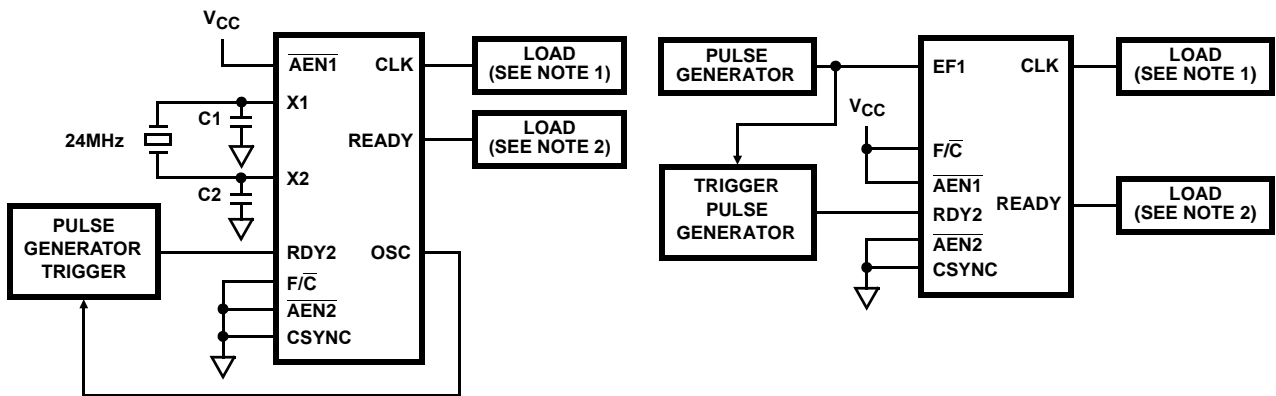
FIGURE 7. TRYLCL, TRYCH LOAD CIRCUITS
