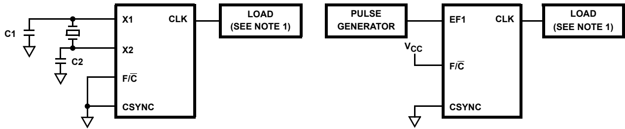
FIGURE 6. TCHCL, TCHCH LOAD CIRCUITS
