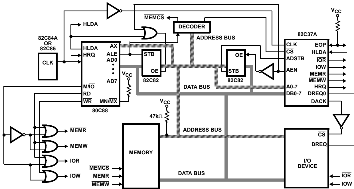
FIGURE 1. APPLICATION FOR DMA SYSTEM
