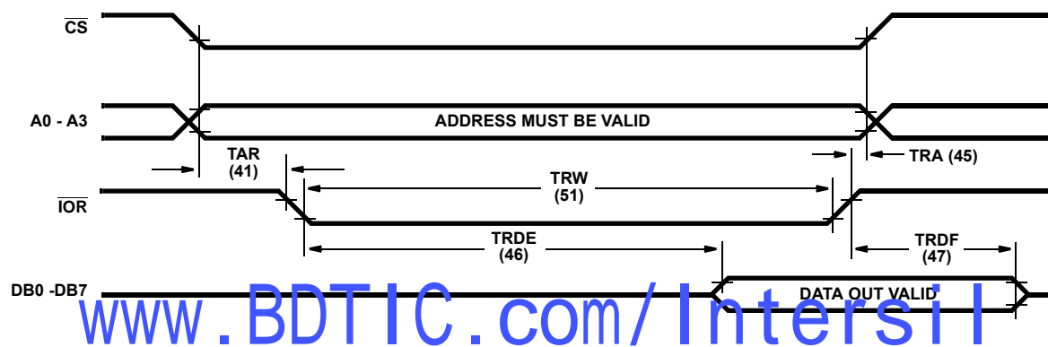
FIGURE 9. SLAVE MODE READ
