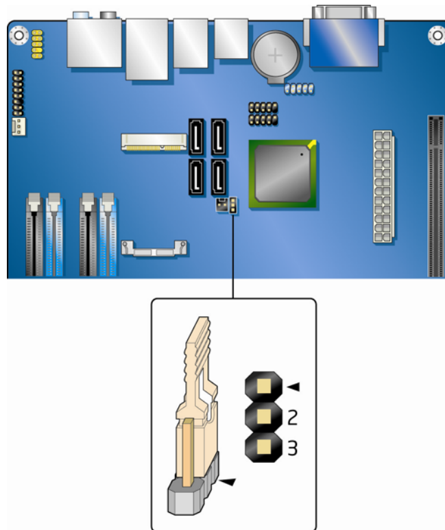
Figure 30. Location of the BIOS Configuration Jumper Block
