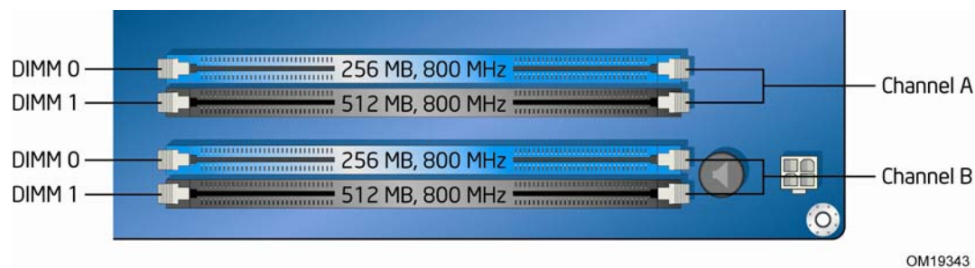
Figure 17. Dual Channel Memory Configuration Example 2
