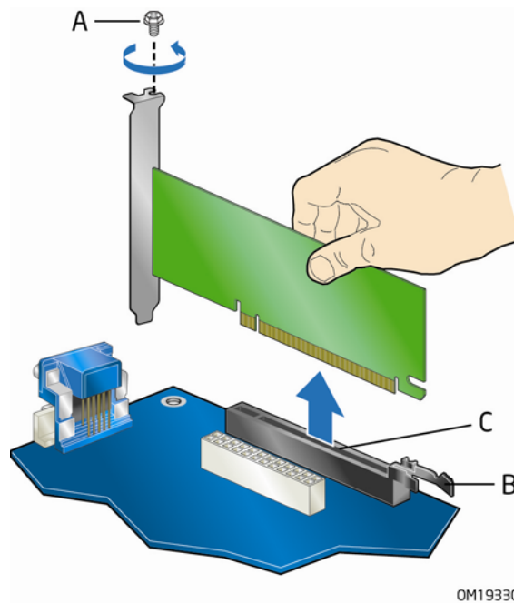
Figure 22. Removing a PCI Express x16 Card
