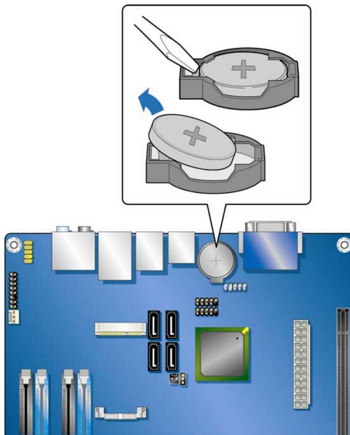
Figure 32. Removing the Battery
