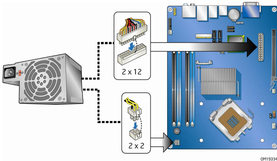
Figure 29. Connecting Power Supply Cables
