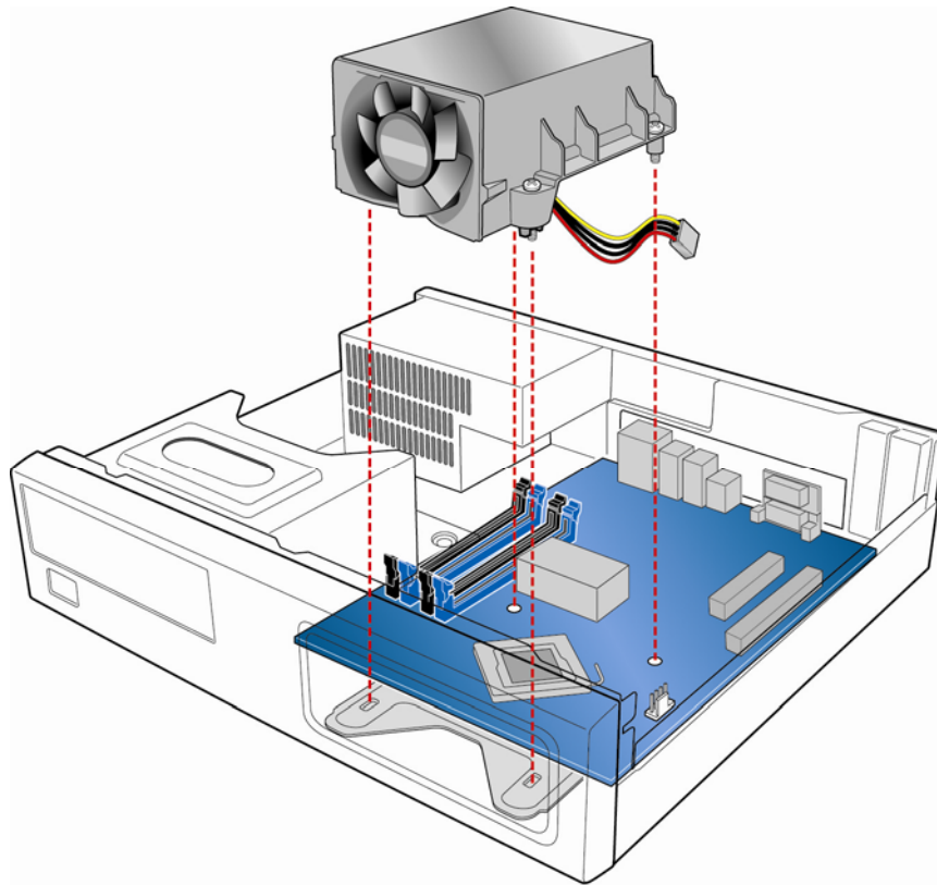
Figure 12. Position the Thermal Module Over the Mounting Holes
