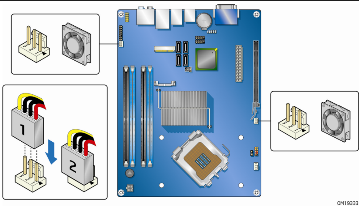
Figure 28. Location of Chassis Fan Headers
