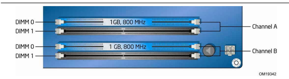
Figure 16. Dual Channel Memory Configuration Example 1
