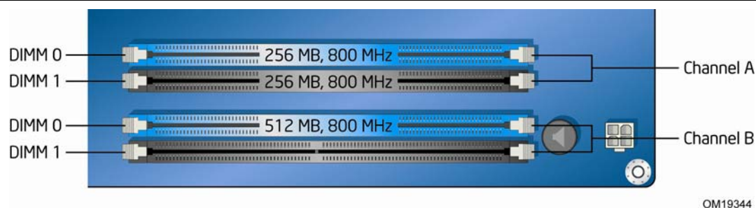
Figure 18. Dual Channel Memory Configuration Example 3
