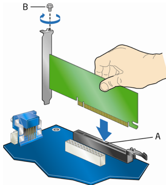
Figure 21. Installing a PCI Express x16 Card
