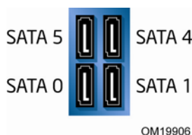
Figure 34. SATA Port Mapping for Desktop Board DG965PZ After RAID is Enabled
