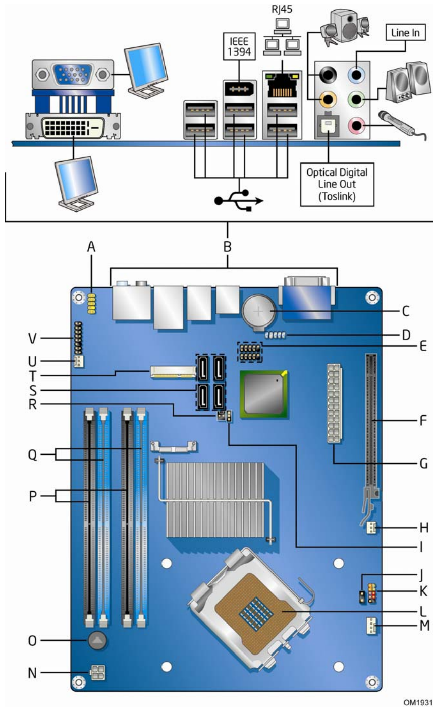
Figure 1. Desktop Board DG965PZ Components
