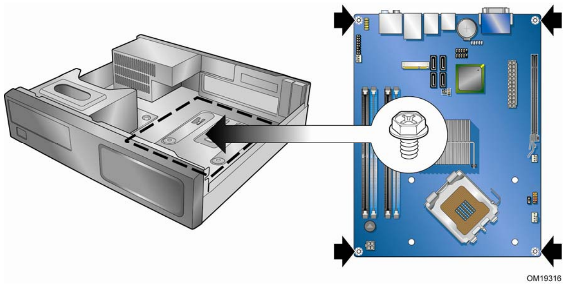
Figure 5. Desktop Board DG965PZ Mounting Screw Hole Locations
