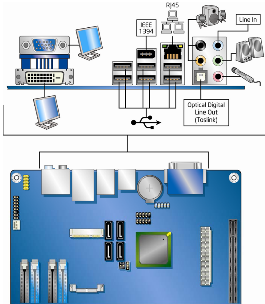
Figure 31. Back Panel Connectors
