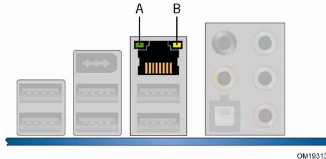
Figure 2. LAN Connector LEDs
