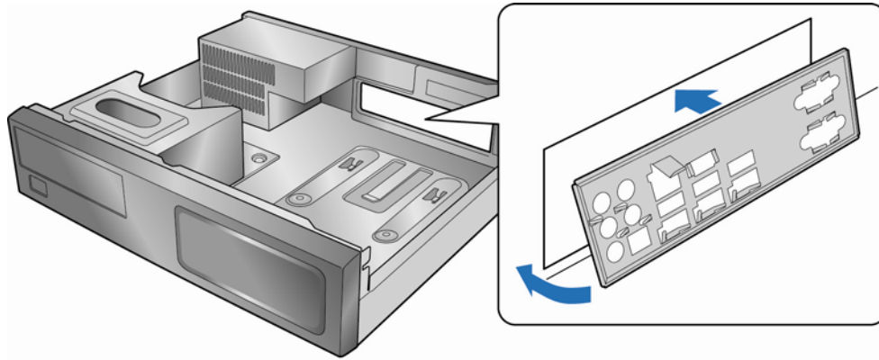
Figure 4. Installing the I/O Shield
