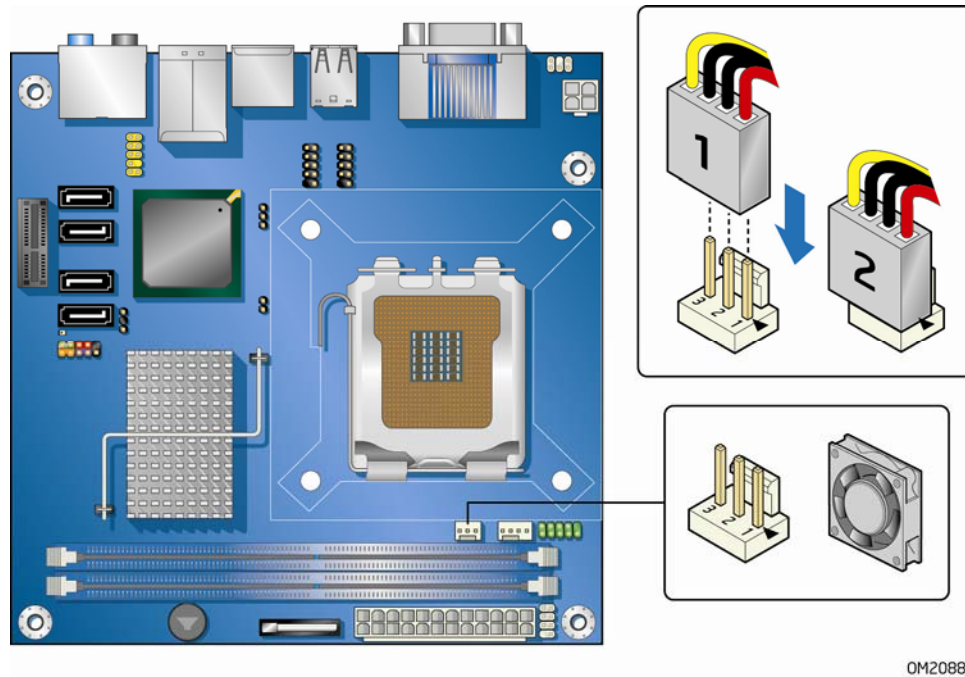
Figure 19. Location of the Chassis Fan Headers
