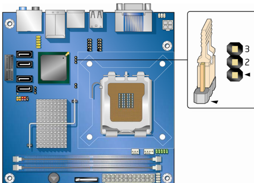
Figure 21. Location of the BIOS Configuration Jumper Block
