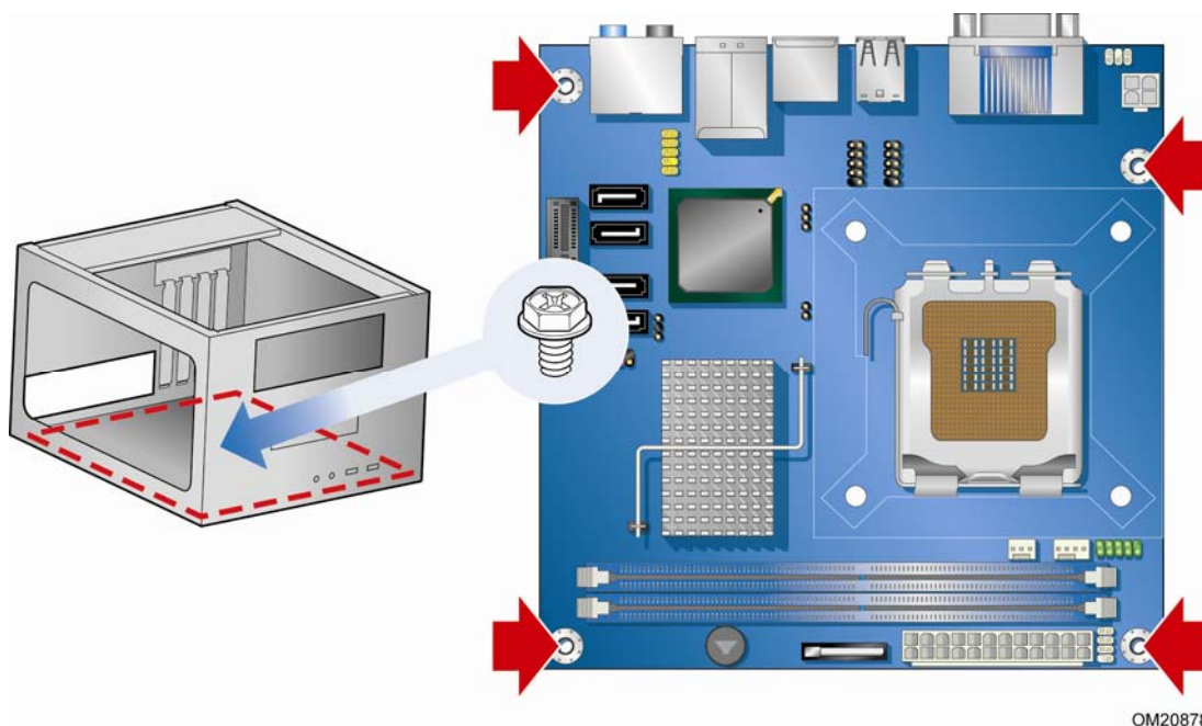
Figure 5. Desktop Board DG45FC Mounting Screw Hole Locations
