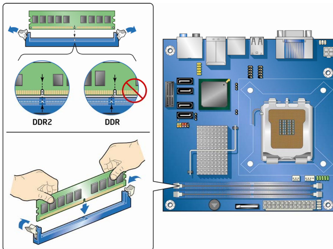
Figure 15. Installing a DIMM
