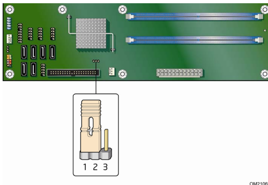
Figure 24. Location of the BIOS Configuration Jumper Block
