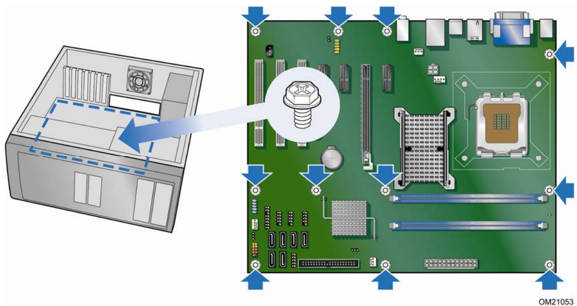
Figure 5. Intel Desktop Board DG43NB Mounting Screw Hole Locations
