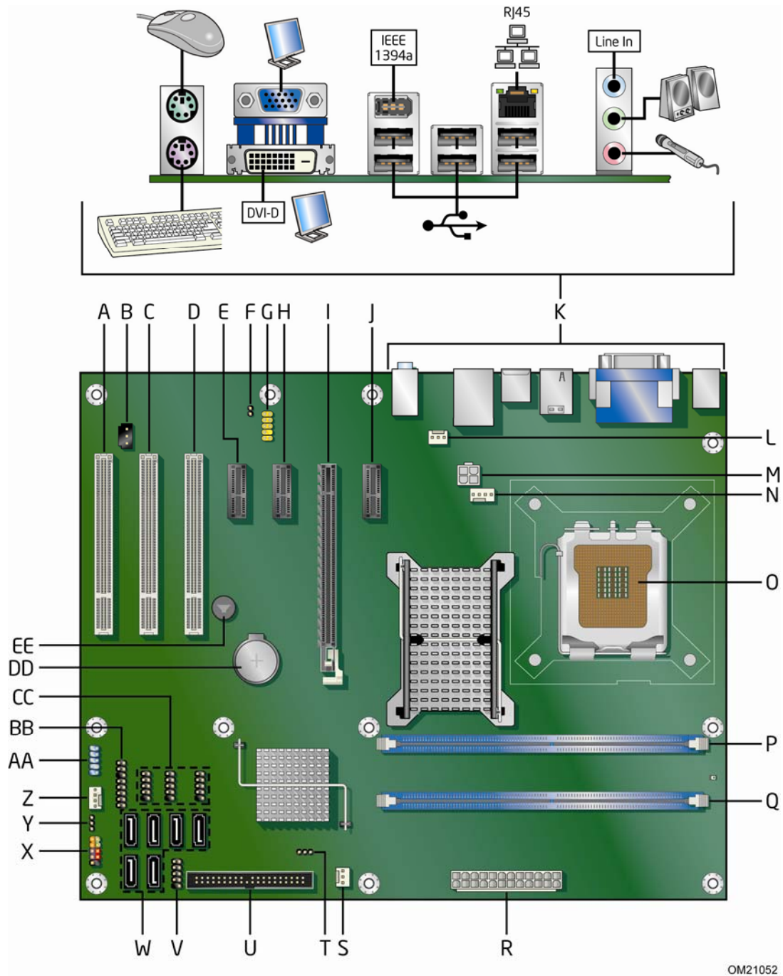
Figure 1. Intel Desktop Board DG43NB Components
