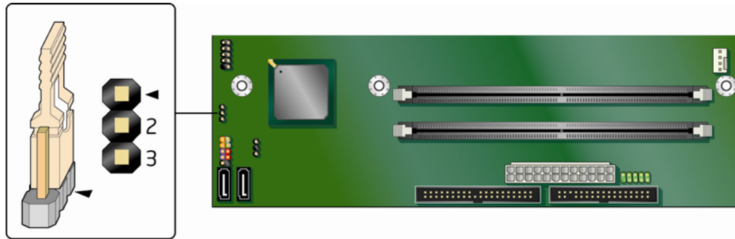
Figure 23. Location of the BIOS Configuration Jumper Block
