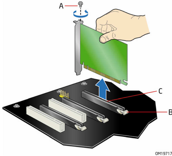
Figure 21. Removing the PCI Express x16 Card
