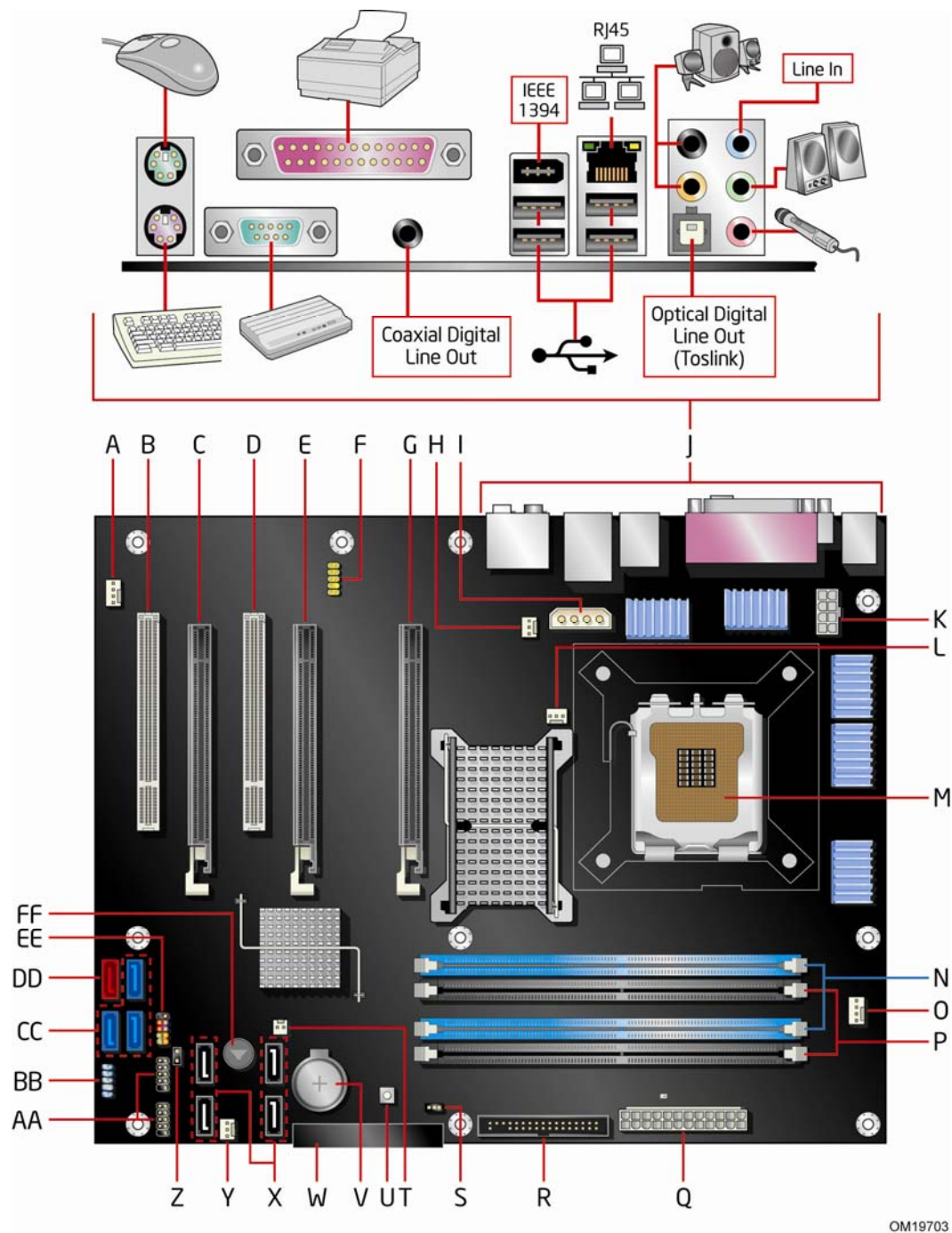
Figure 1. Desktop Board D975XBX2 Components
