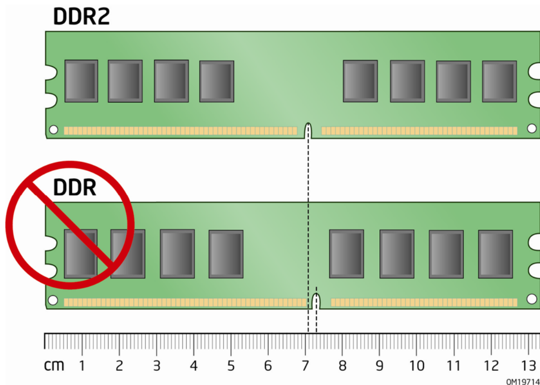
Figure 17. Use DDR2 DIMMs
