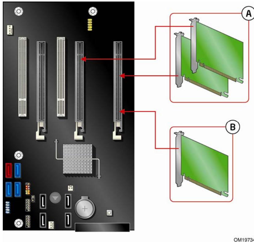
Figure 19. Installing PCI Express Graphics Cards
