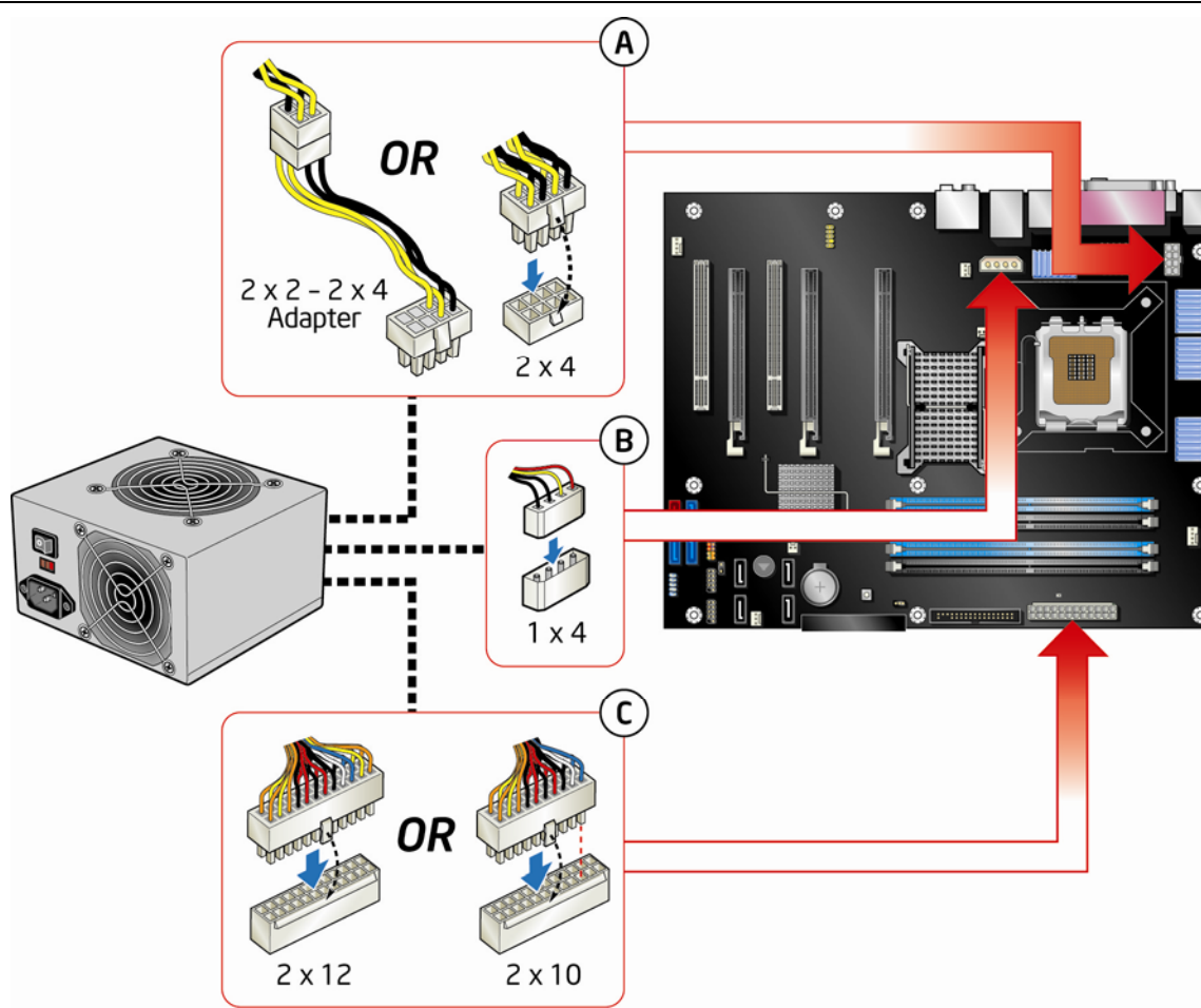
Figure 28. Connecting Power Supply Cables
