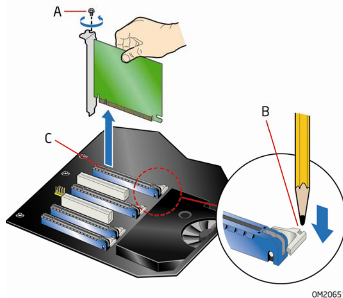
Figure 20. Removing a PCI Express x16 Card
