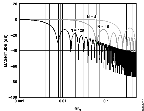
Figure 21. Frequency Response—Moving Average Filter
