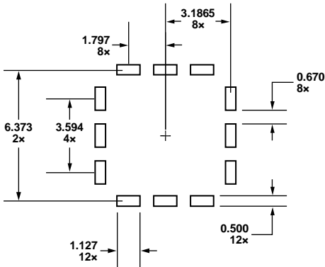
7.2mm x 7.2mm STACKED LGA. ALL DIMENSIONS IN mm. Figure 5. Second-Level Assembly Pad Layout
