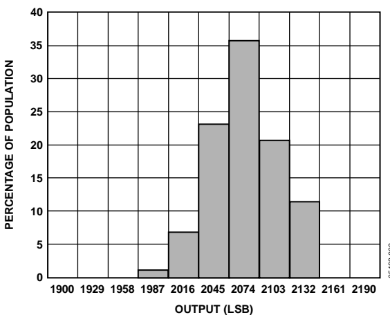
Figure 10. X-Axis Zero g Bias at 25°C
