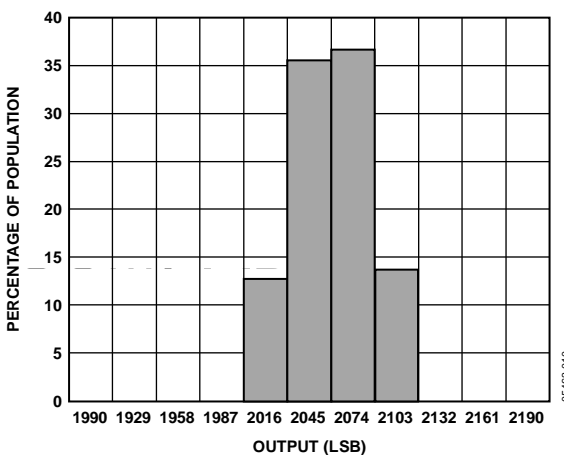
Figure 11. Y-Axis Zero g Bias at 25°C
