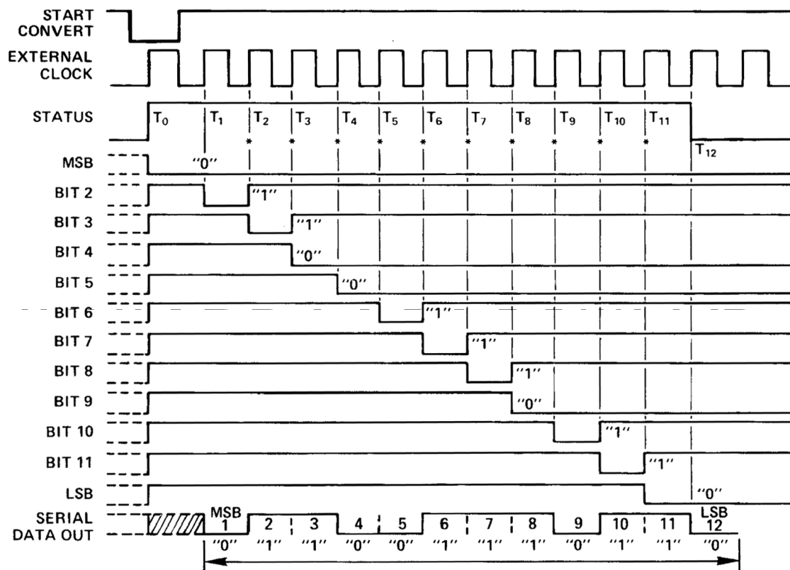
Figure 3. Timing Diagram
