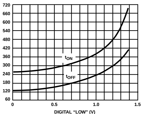
FIGURE 13. SWITCHING TIMES FOR NEGATIVE DIGITAL TRANSITION
