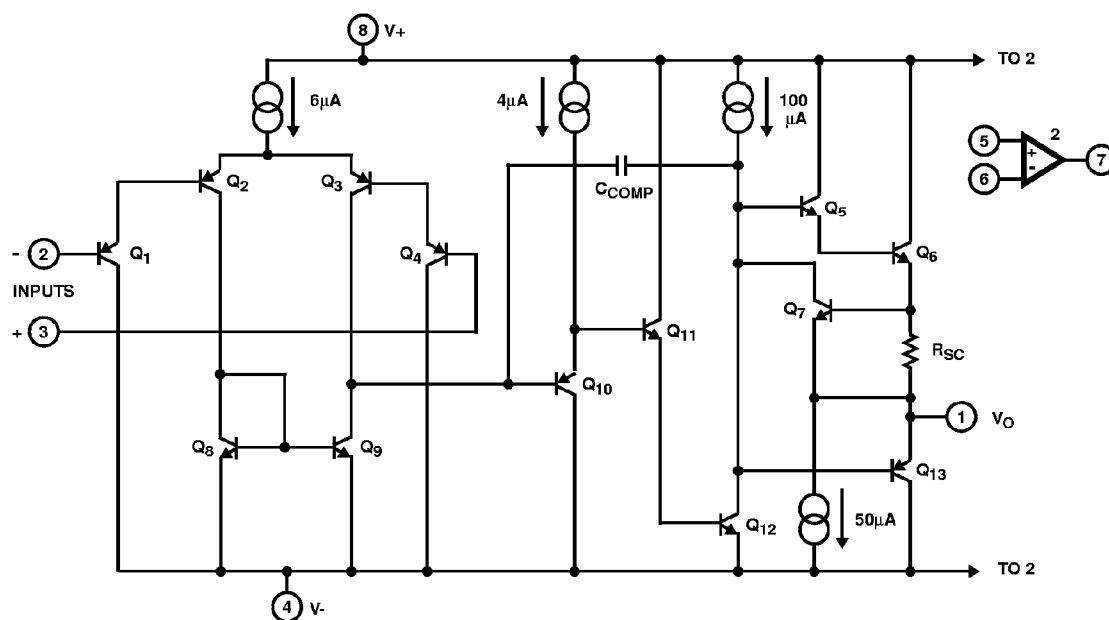
ONE OF TWO OPERATIONAL AMPLIFIERS
