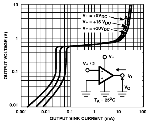
FIGURE 12. OUTPUT SINK CURRENT CHARACTERISTICS
