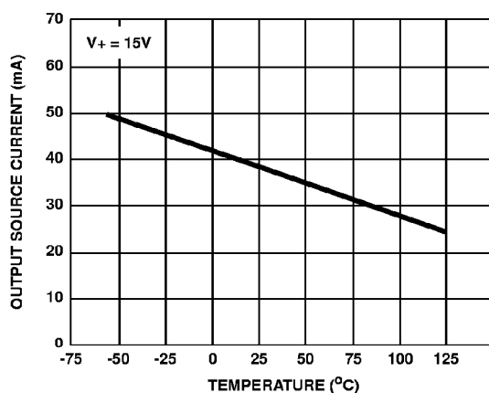
FIGURE 13. OUTPUT CURRENT vs AMBIENT TEMPERATURE
