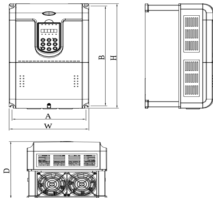
图2-3 EV5000-4T0022G~EV5000-4T0220G
