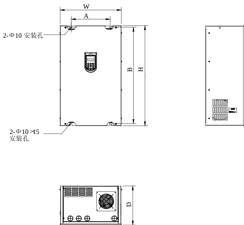
图2-4 EV5000-4T0300G~EV5000-4T2200G
