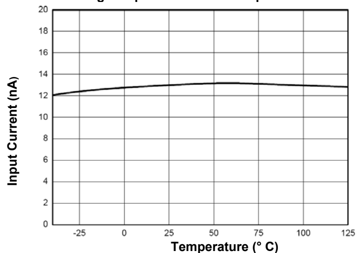
Fig.2- Input Current vs. Temperature
