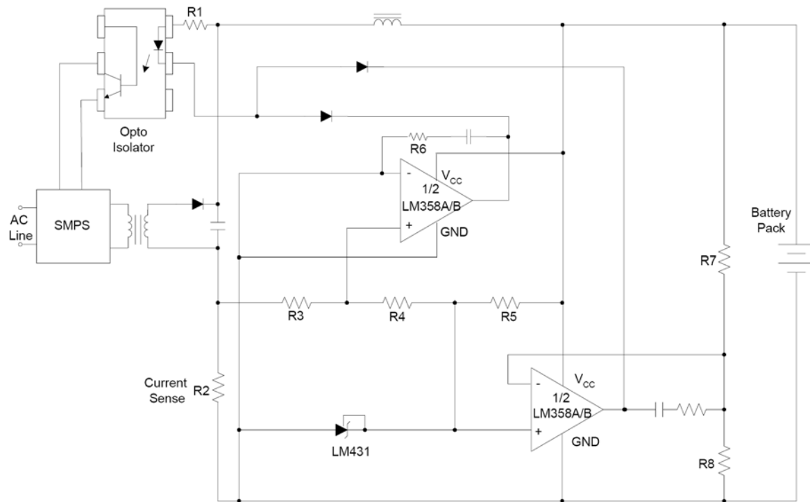
Fig.13- Battery Charger
